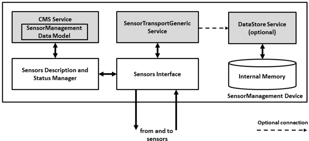
Figure 1 — IOT Management and Control Device Functional Diagram
